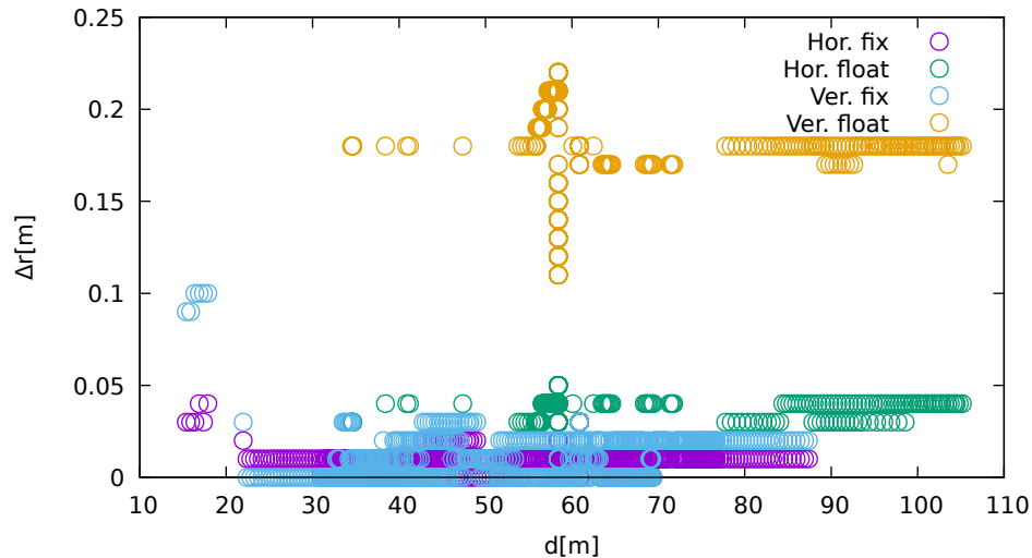
displacement vs distance (LeicaGS15 at C_1 )
