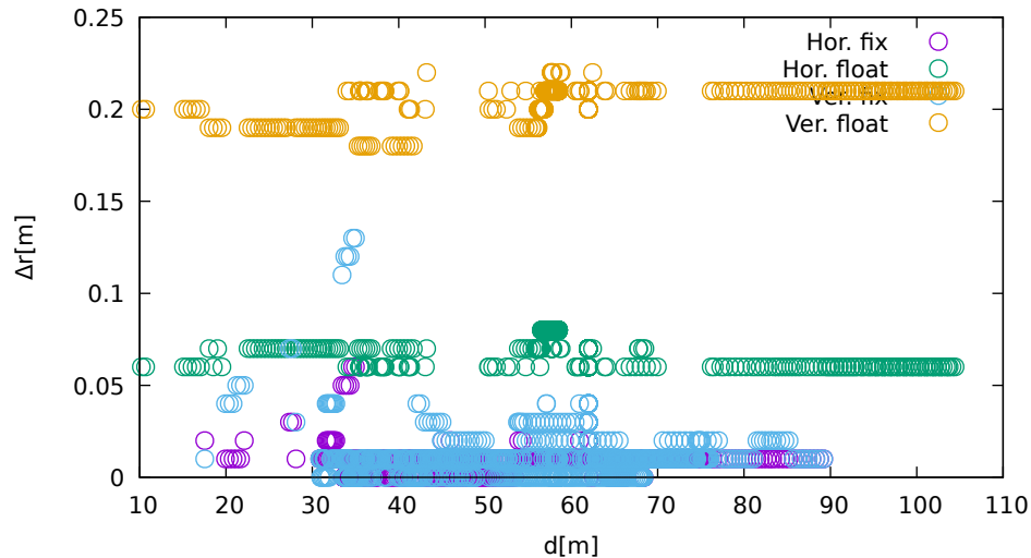
displacement vs distance (LeicaGS18 at C_1 )
