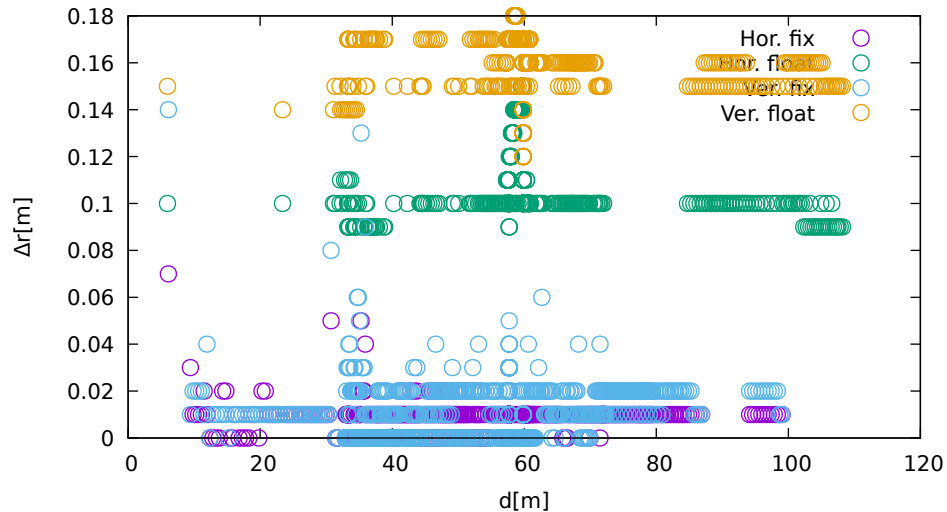
displacement vs distance (TrimbleR8s at C 1 )
