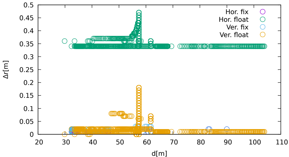
displacement vs distance (ublox9 at C 1 )
