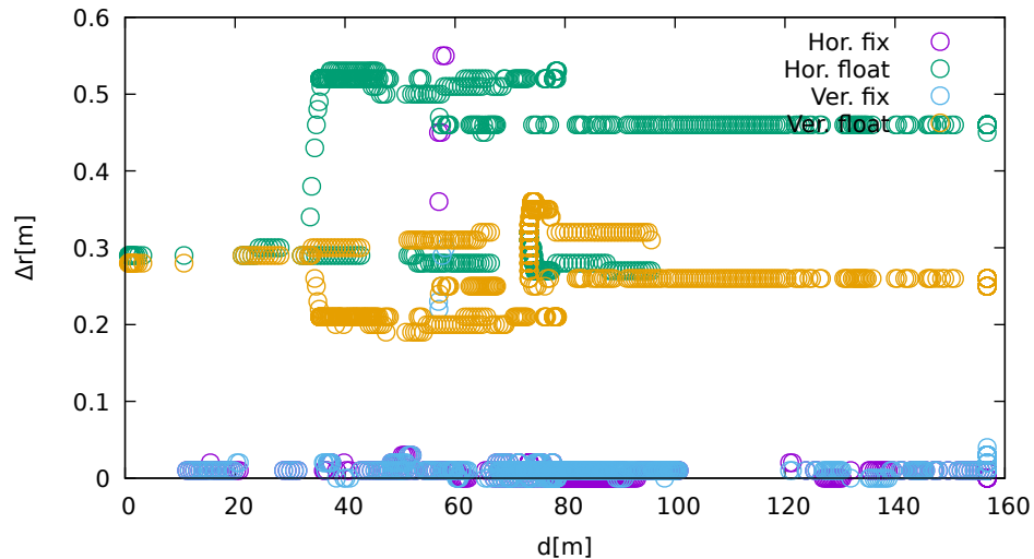
displacement vs distance (JavadLSA at C 2 )
