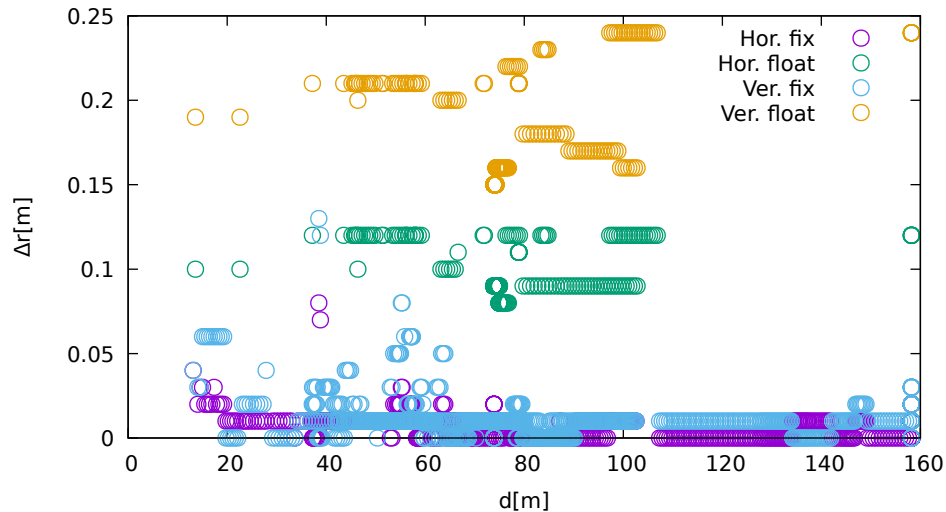
displacement vs distance (LeicaGS15 at C 2 )
