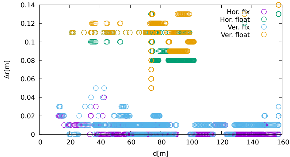
displacement vs distance (LeicaGS18 at C 2 )
