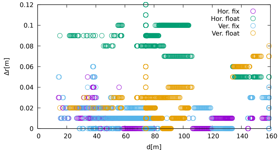
displacement vs distance (TrimbleR10 at C 2 )
