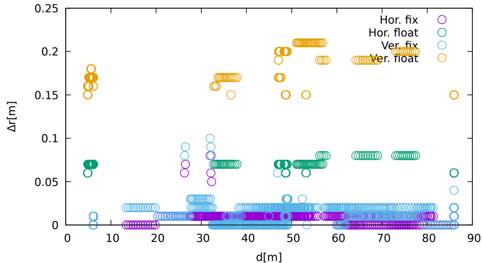
displacement vs distance (LeicaGS15 at C 3 )
