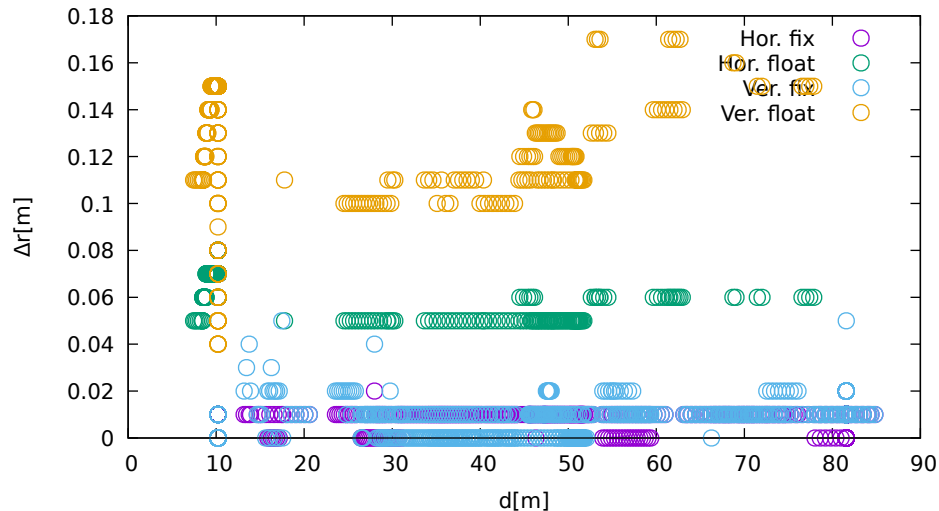
displacement vs distance (LeicaGS18 at C 3 )
