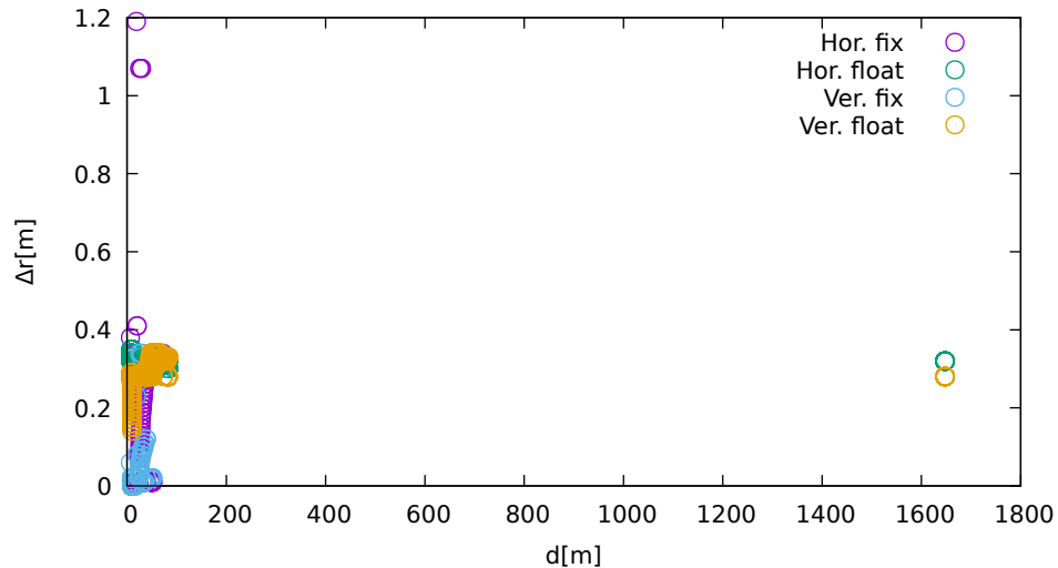
displacement vs distance (ublox at C 3 )
