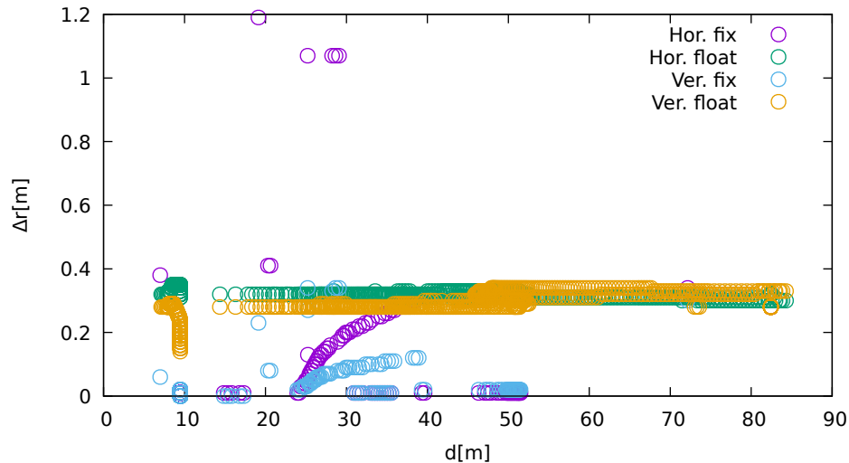
displacement vs distance (ublox9 at C 3 )
