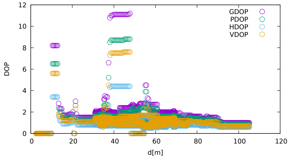
DOP vs distance (LeicaGS15 at C 1 )
