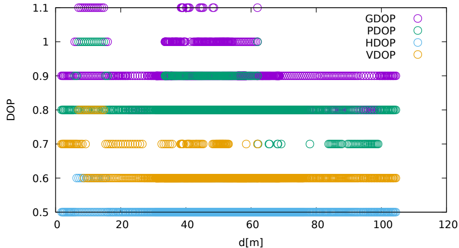
DOP vs distance (LeicaGS18 at C 1 )
