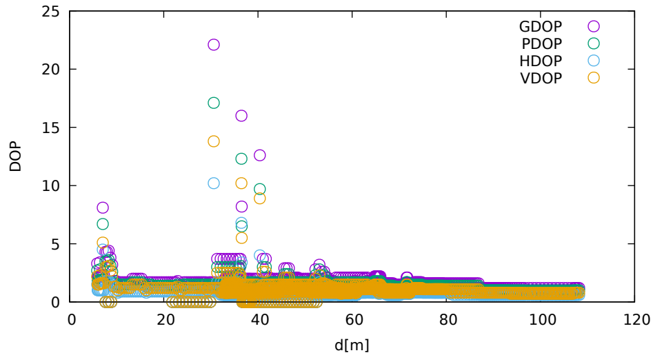
DOP vs distance (TrimbleR8s at C 1 )
