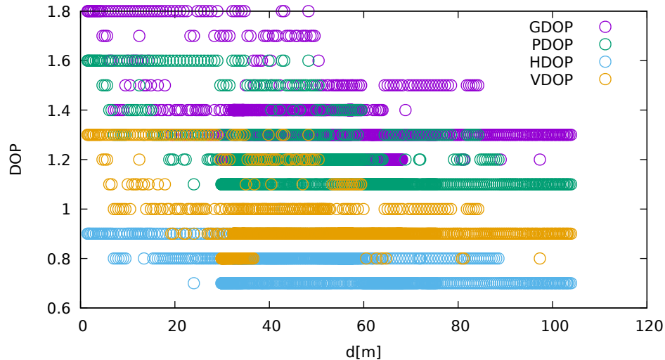
DOP vs distance (ublox9 at C 1 )
