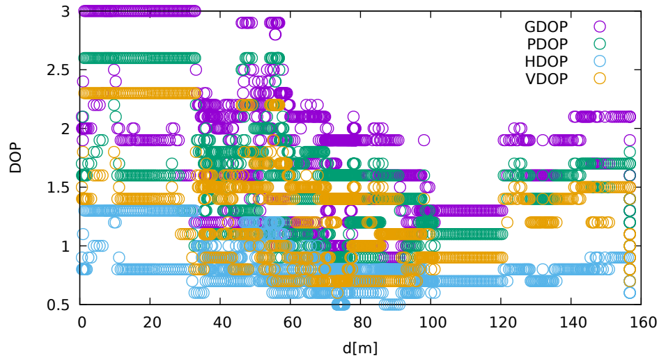
DOP vs distance (JavadLSA at C 2 )
