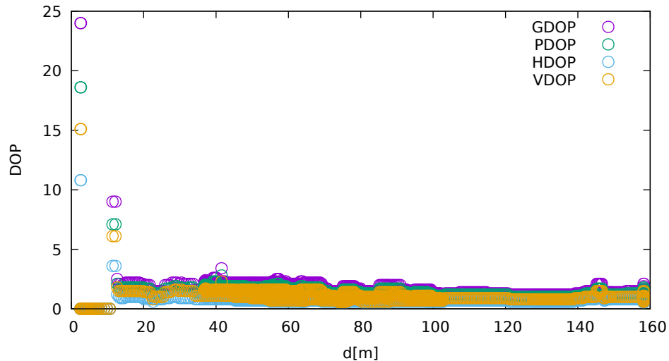
DOP vs distance (LeicaGS15 at C 2 )
