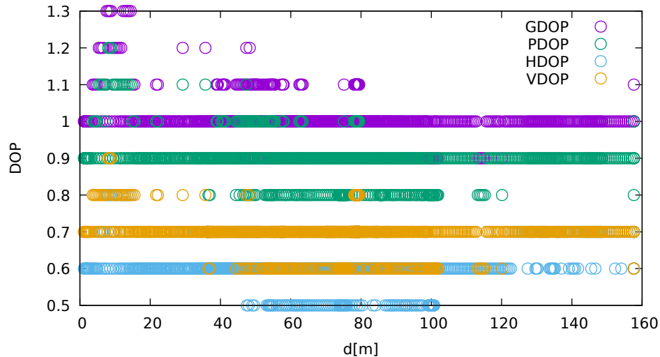
DOP vs distance (LeicaGS18 at C 2 )
