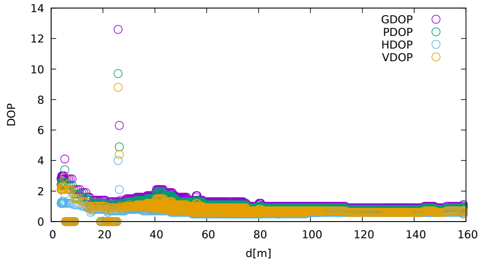
DOP vs distance (TrimbleR10 at C 2 )
