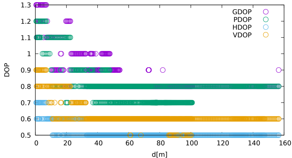
DOP vs distance (ublox9 at C 2 )
