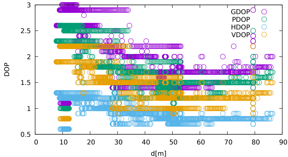
DOP vs distance (JavadLSA at C 3 )
