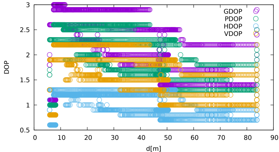
DOP vs distance (JavadVS at C 3 )
