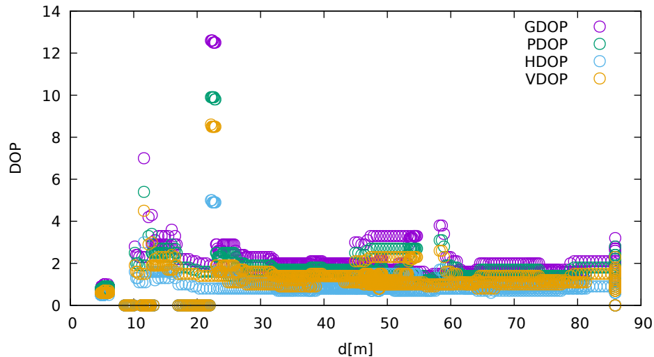
DOP vs distance (LeicaGS15 at C 3 )
