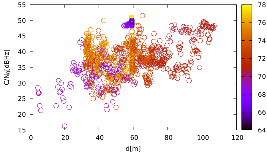
C/N 0 vs distance (JavadLSA at C 1 for G01 at L2)
