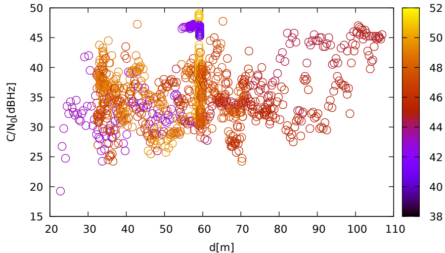
C/N 0 vs distance (JavadLSA at C 1 for G03 at L2)
