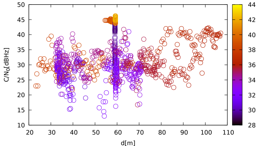
C/N 0 vs distance (JavadLSA at C 1 for G08 at L2)
