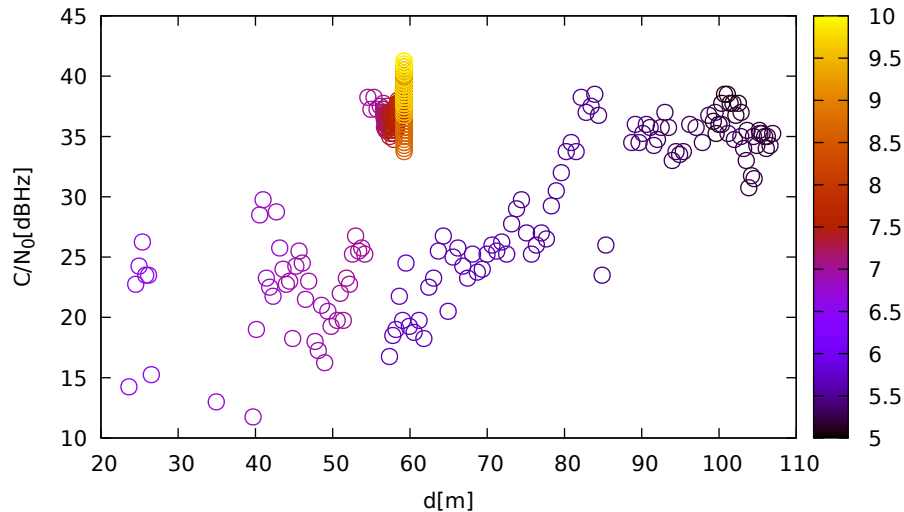
C/N 0 vs distance (JavadLSA at C 1 for G10 at L2)
