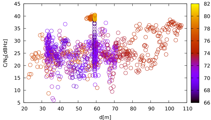
C/N 0 vs distance (JavadLSA at C 1 for G11 at L2)
