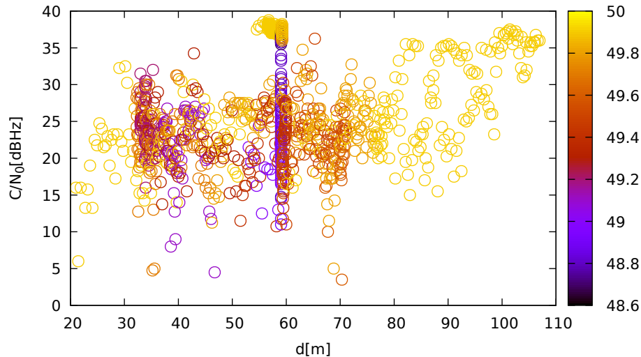
C/N 0 vs distance (JavadLSA at C 1 for G14 at L2)
