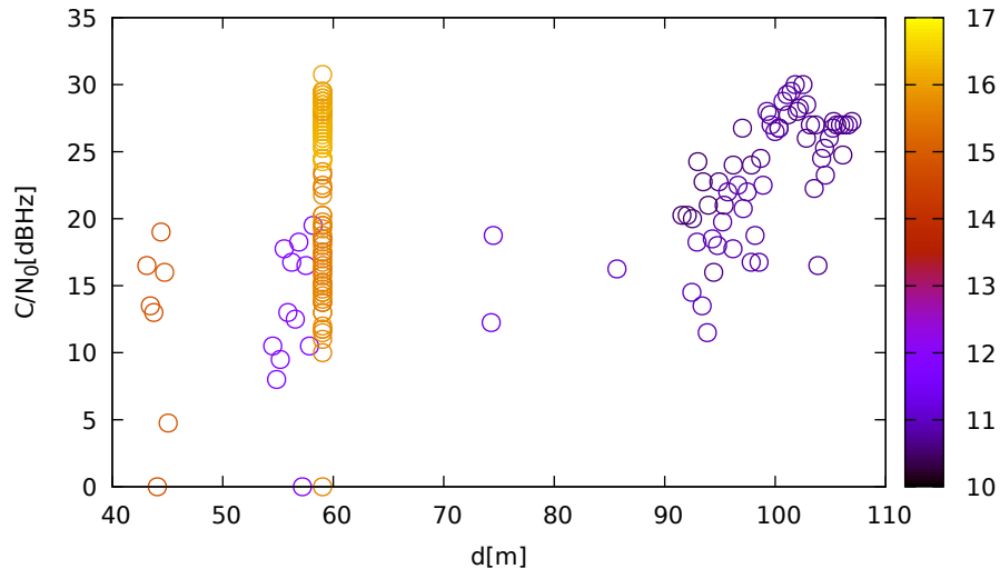
C/N 0 vs distance (JavadLSA at C 1 for G17 at L2)
