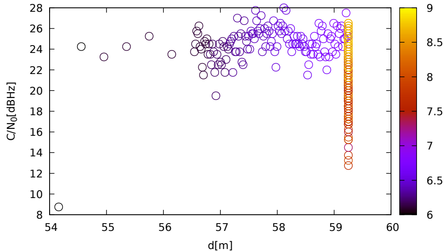
C/N 0 vs distance (JavadLSA at C 1 for G21 at L2)
