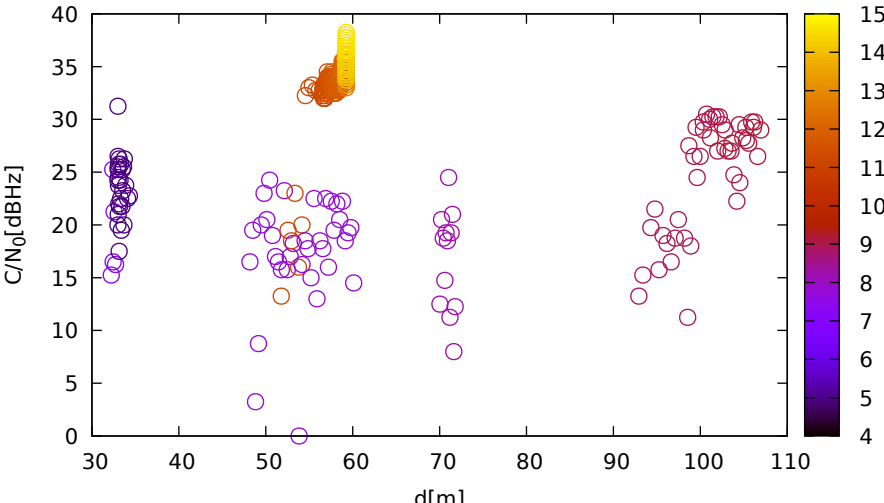
C/N 0 vs distance (JavadLSA at C 1 for G27 at L2)
