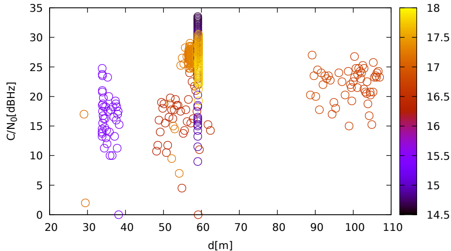
C/N 0 vs distance (JavadLSA at C 1 for G28 at L2)
