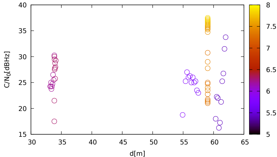
C/N 0 vs distance (JavadLSA at C 1 for G31 at L2)
