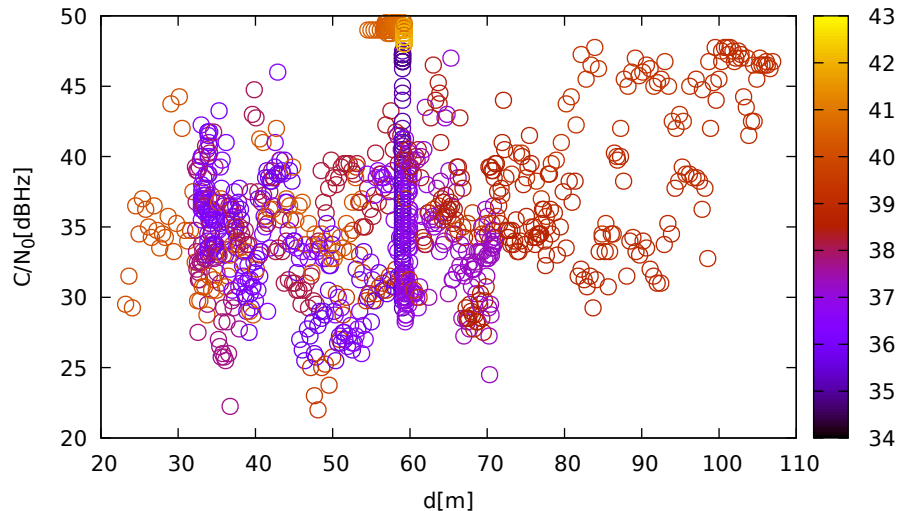
C/N 0 vs distance (JavadLSA at C 1 for G32 at L2)
