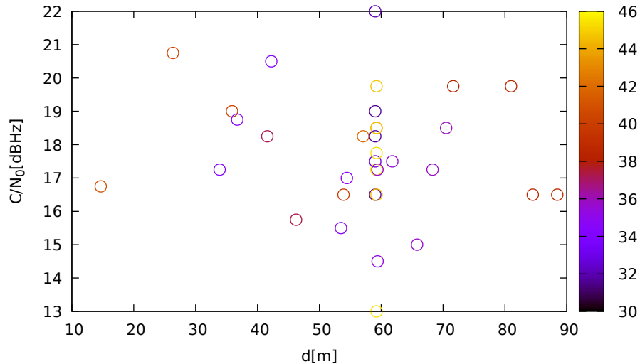
C/N 0 vs distance (JavadLSA at C 1 for R06 at L2)
