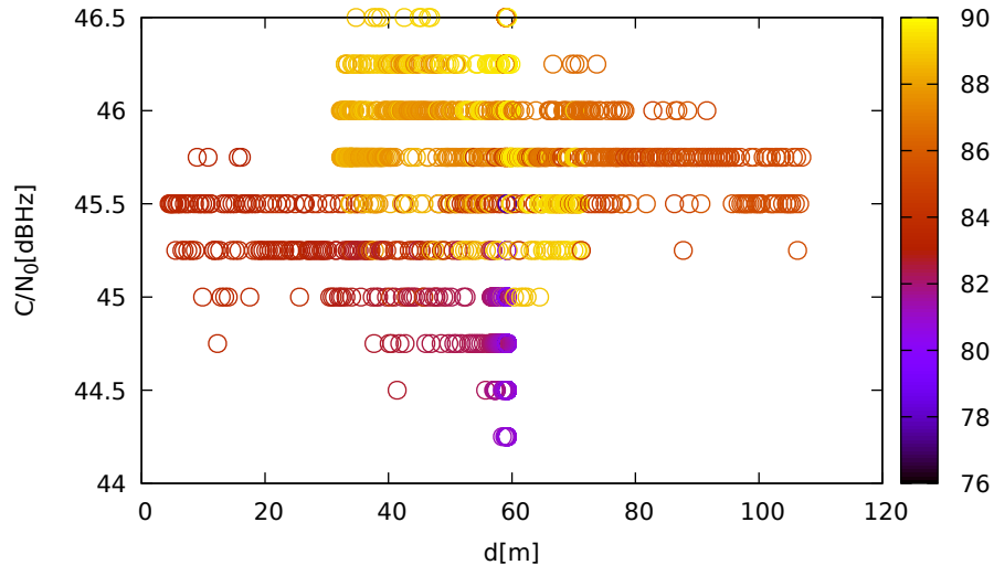
C/N 0 vs distance (JavadLSA at C 1 for R07 at L2)
