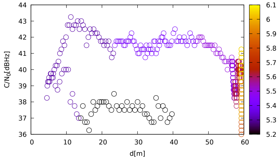
C/N 0 vs distance (JavadLSA at C 1 for R14 at L2)
