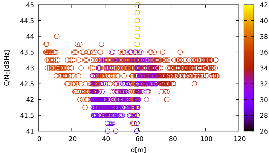
C/N 0 vs distance (JavadLSA at C 1 for R21 at L2)
