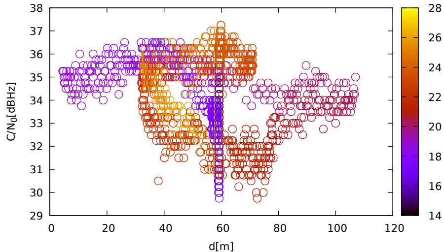
C/N 0 vs distance (JavadLSA at C 1 for R23 at L2)
