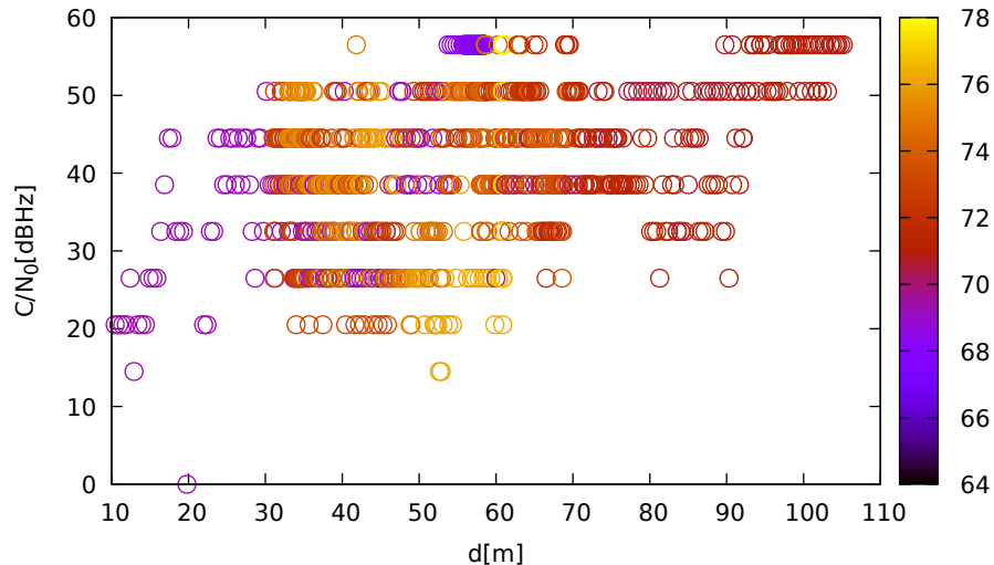
C/N 0 vs distance (LeicaGS15 at C 1 for G01 at L2)
