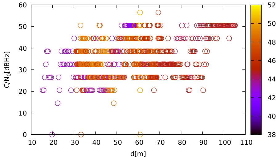
C/N 0 vs distance (LeicaGS15 at C 1 for G03 at L2)
