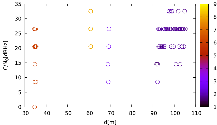
C/N 0 vs distance (LeicaGS15 at C 1 for G04 at L2)
