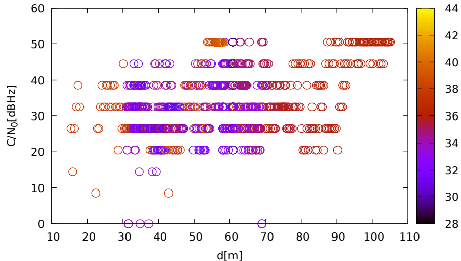
C/N 0 vs distance (LeicaGS15 at C 1 for G08 at L2)
