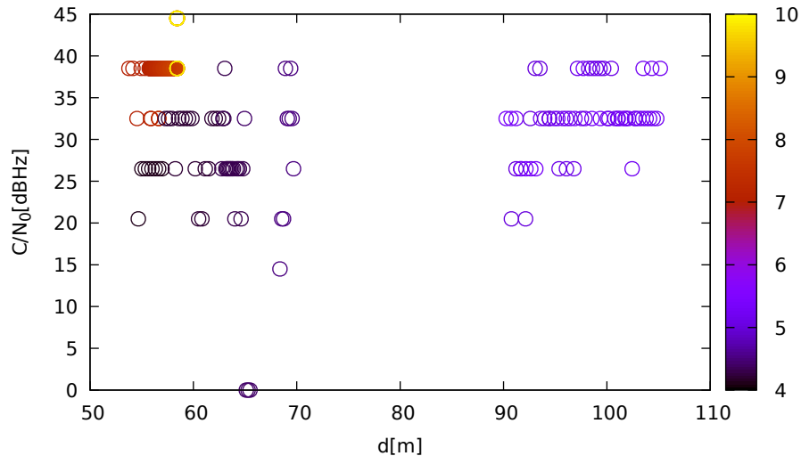
C/N 0 vs distance (LeicaGS15 at C 1 for G10 at L2)
