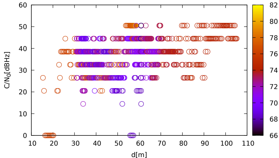
C/N 0 vs distance (LeicaGS15 at C 1 for G11 at L2)
