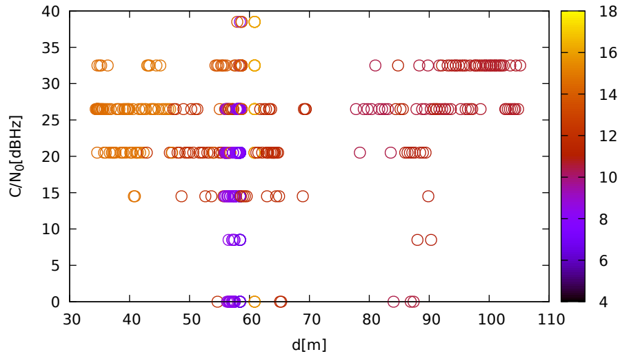
C/N 0 vs distance (LeicaGS15 at C 1 for G17 at L2)
