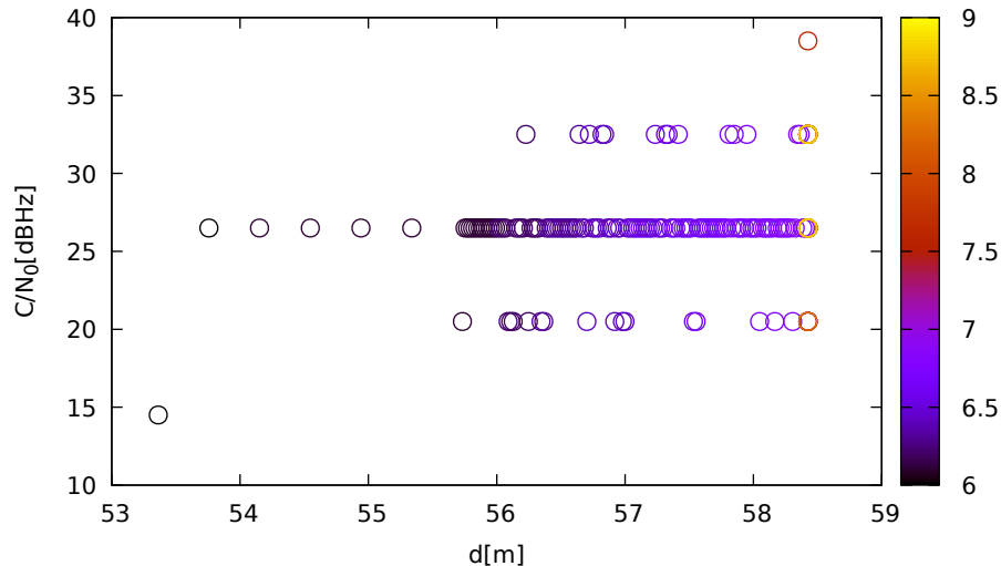
C/N 0 vs distance (LeicaGS15 at C 1 for G21 at L2)
