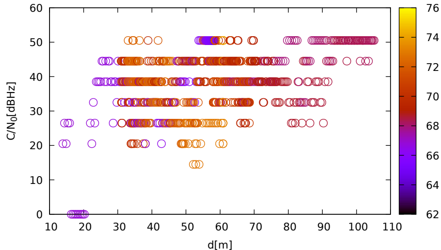
C/N 0 vs distance (LeicaGS15 at C 1 for G22 at L2)
